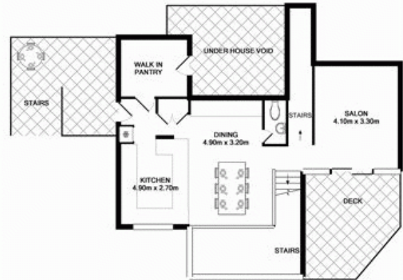
2ND LEVEL APPROX. FLOOR AREA 68.8 SQ.M. (739 SQ.FT.)
