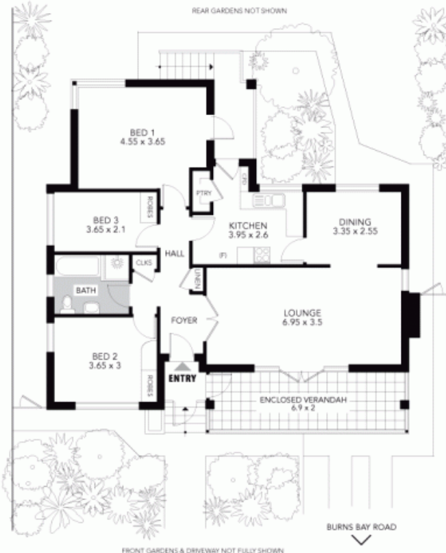
MAIN PLAN: GROUND FLOOR
