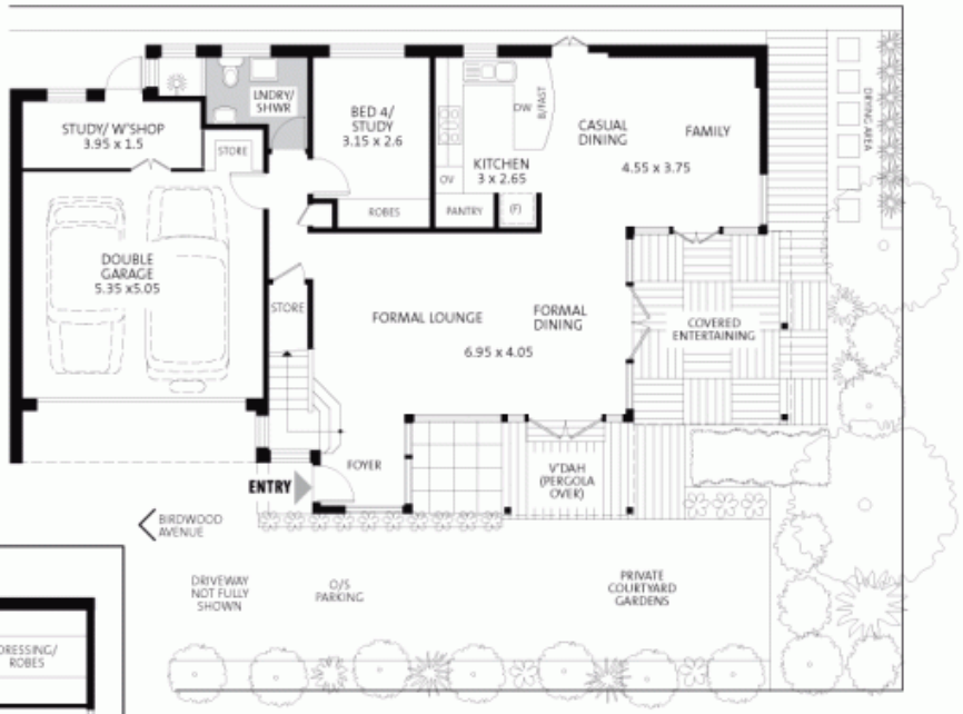
MAIN PLAN: GROUND FLOOR
