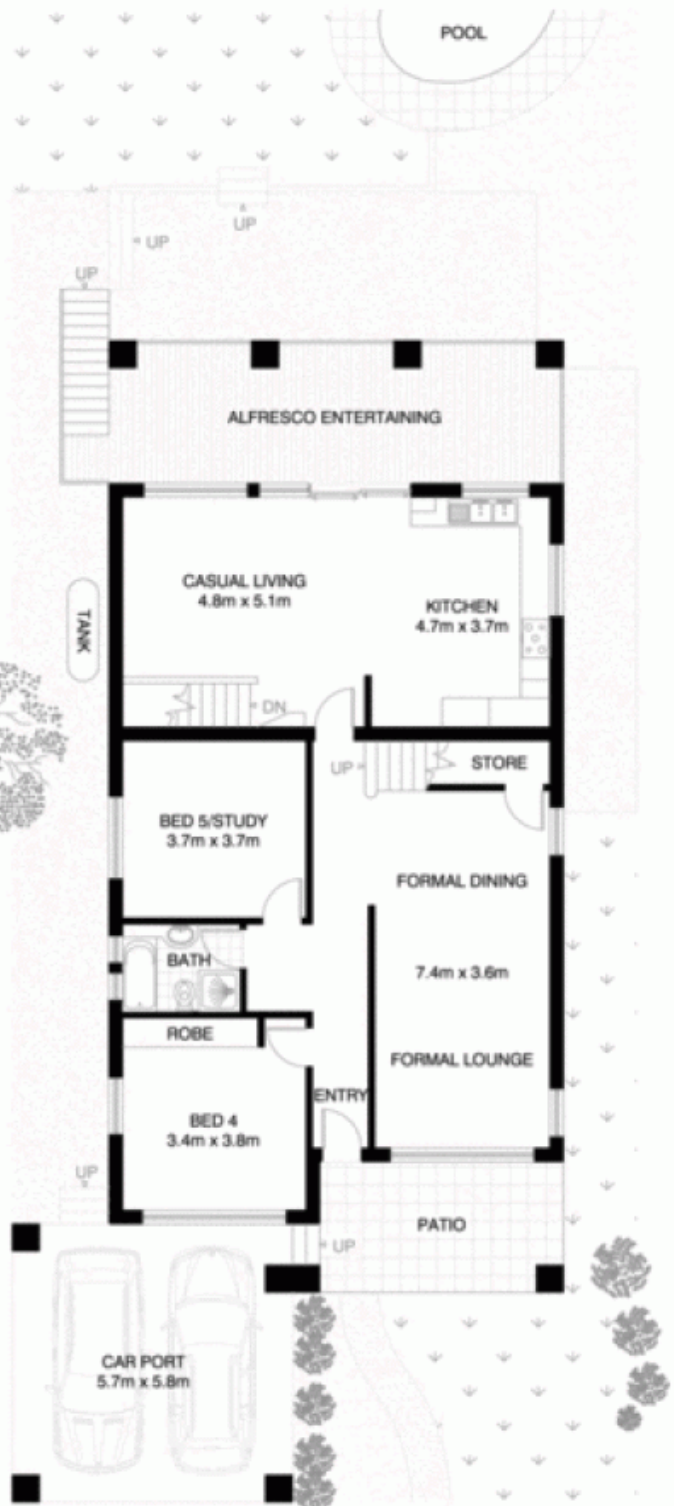
GROUND FLOOR
