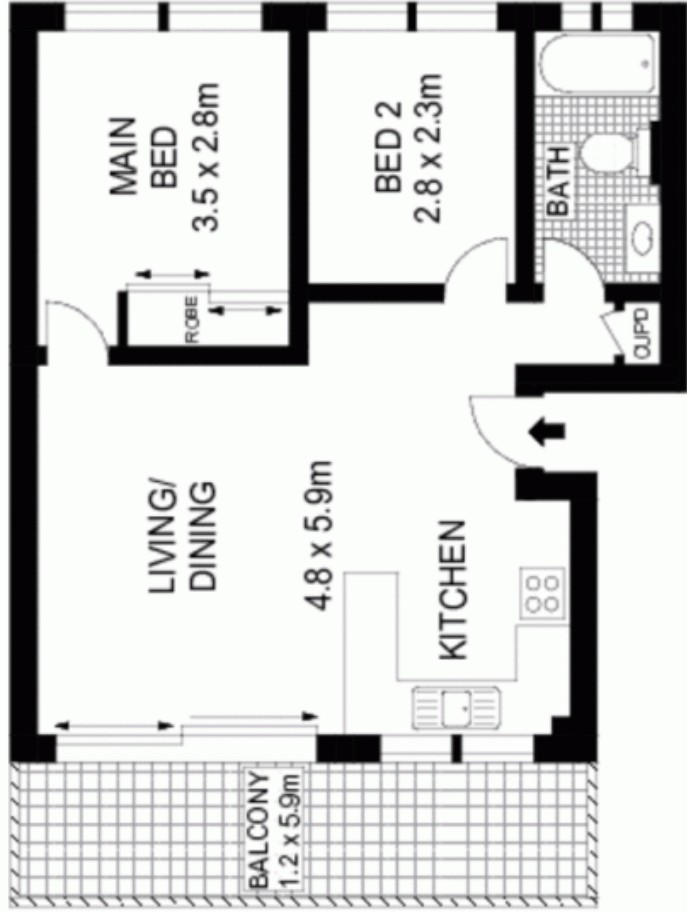
LEVEL TWO
