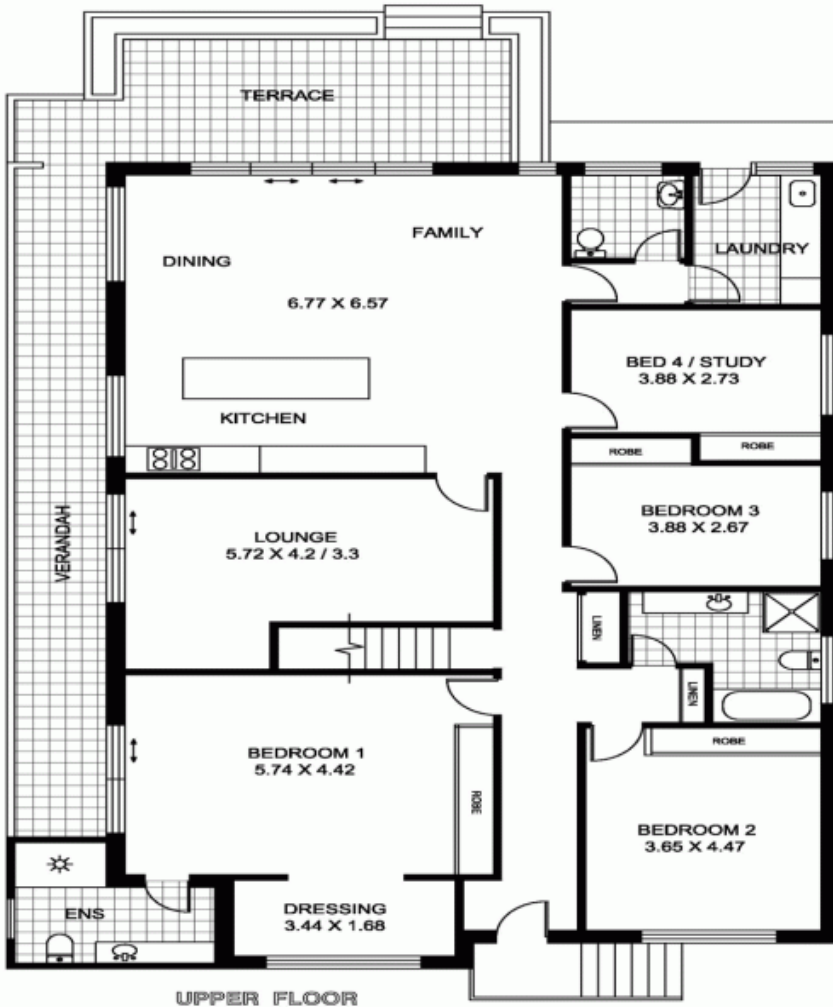
UPPER FLOOR
