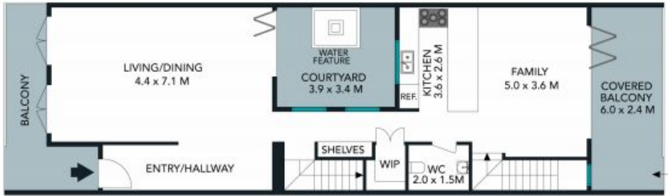
GROUND FLOOR
