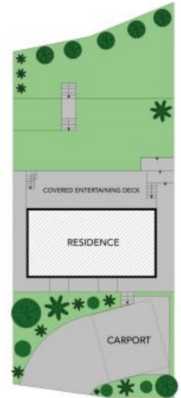
SITE PLAN
