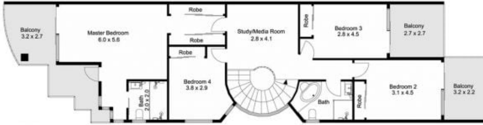
First Floor
