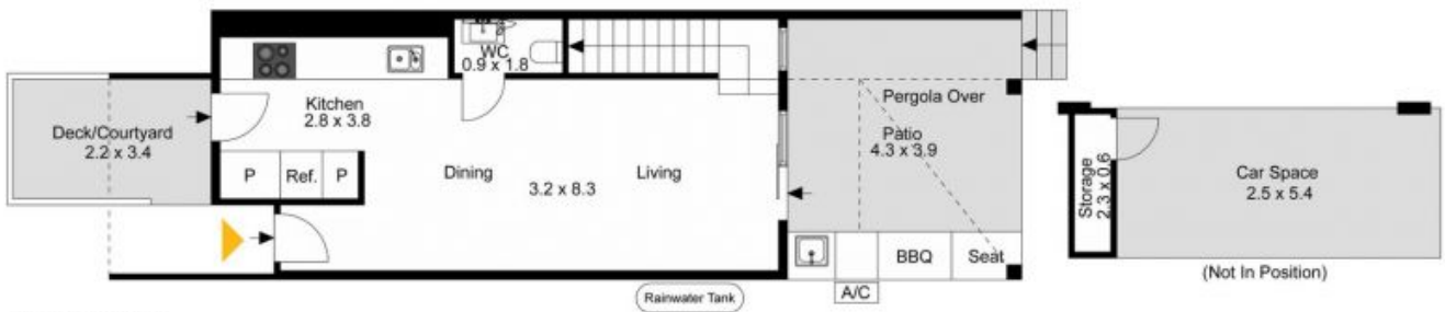
Ground Floor
