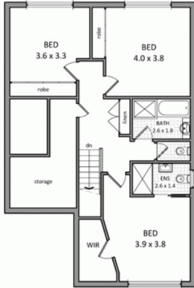
FIRST LEVEL FLOOR PLAN
