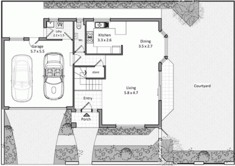
Ground level floor plan
