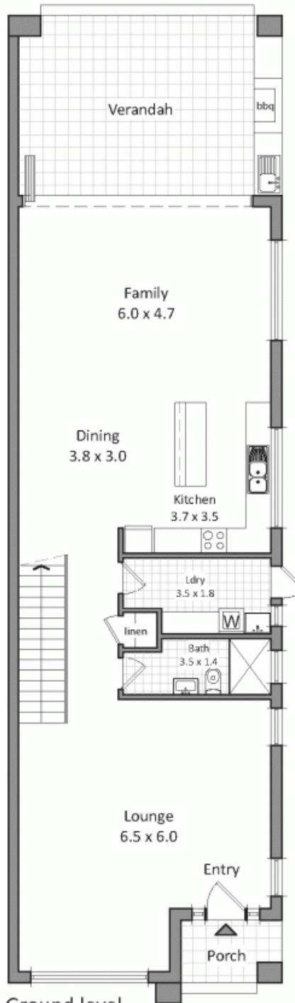
Ground level floor plan
