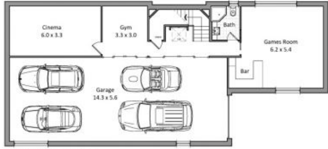
Basement level floor plan
