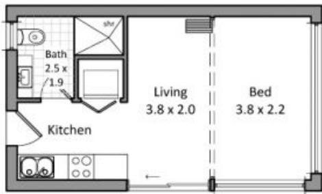
Granny flat floor plan
