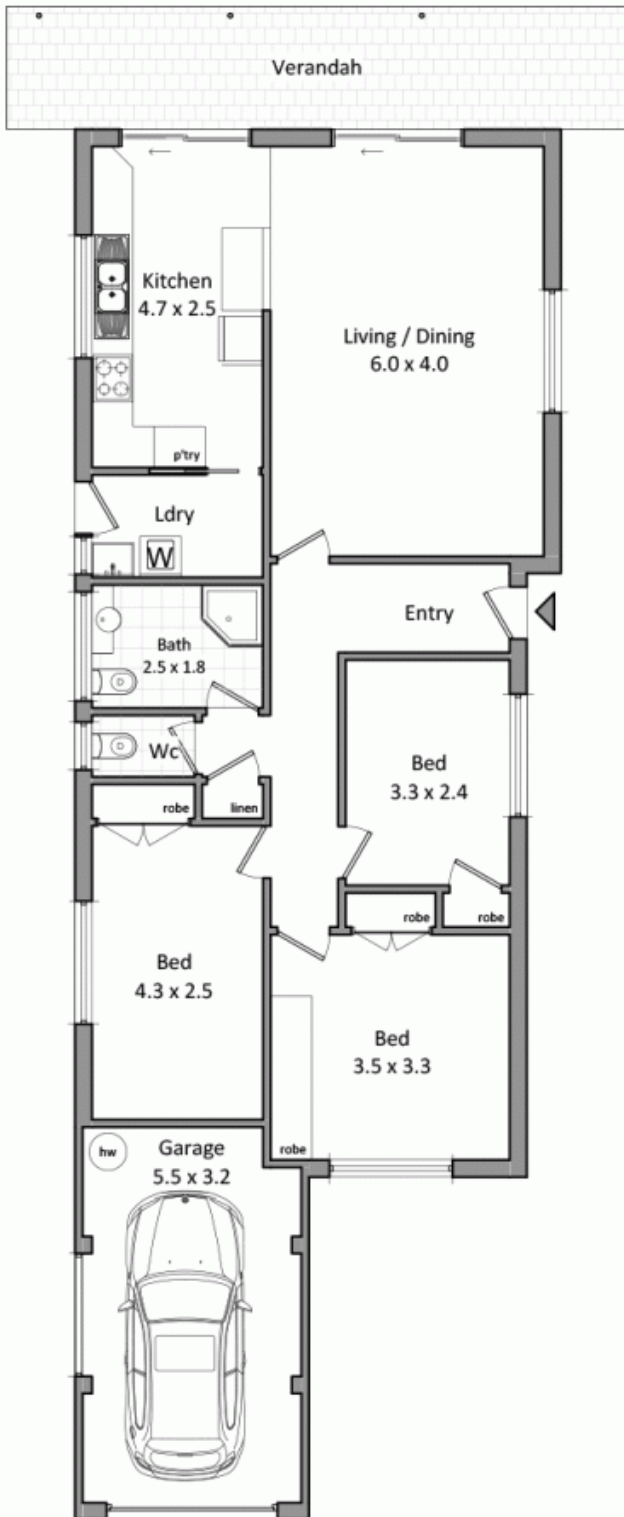
Floor plan
