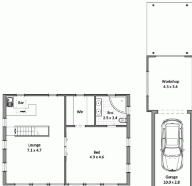
First level floor plan
