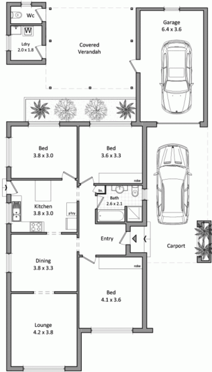
Floor plan
