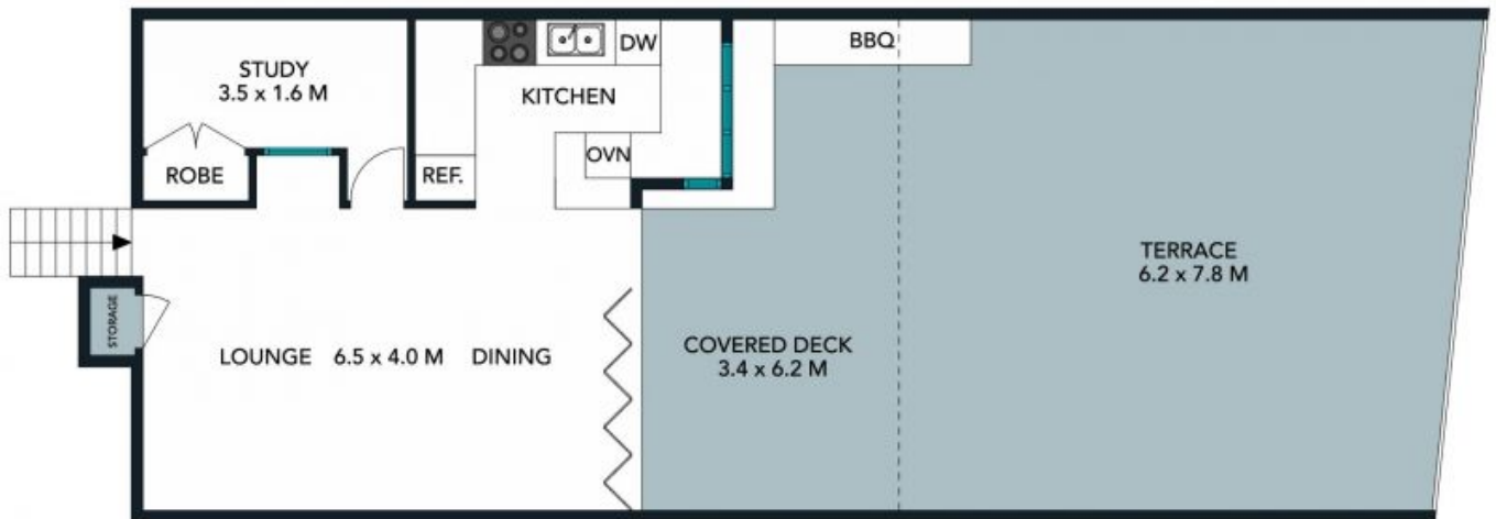
LEVEL 1
