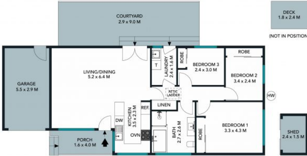
FLOOR PLAN
