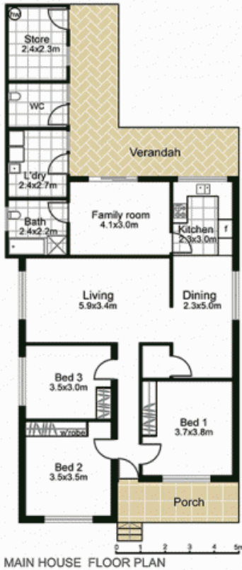
MAIN HOUSE FLOOR PLAN
