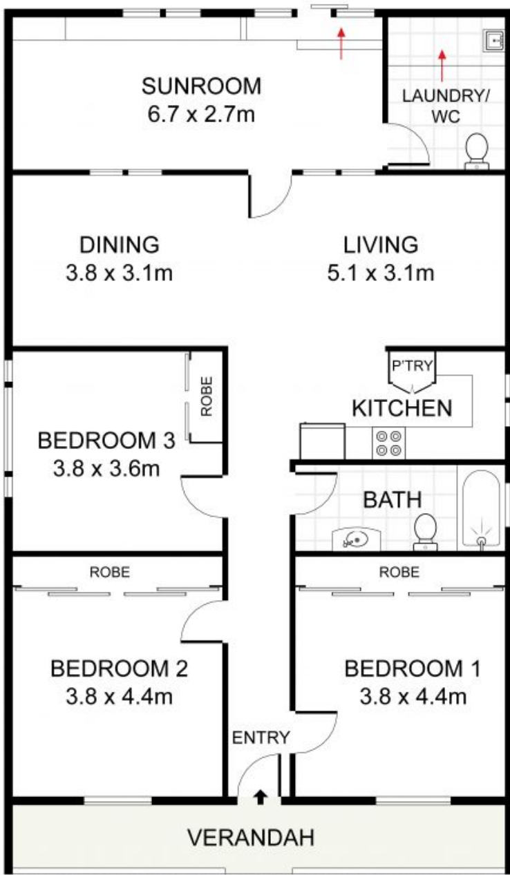
GROUND FLOOR
