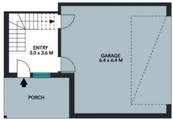
LOWER FLOOR
