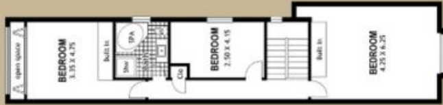
FIRST FLOOR
