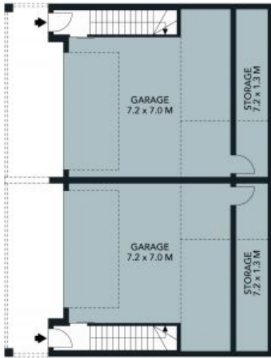
UNITS 3 & 4 GROUND FLOOR PLAN
