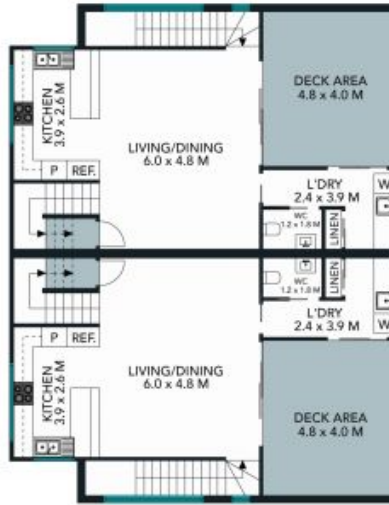
UNITS 3 & 4 FIRST FLOOR
