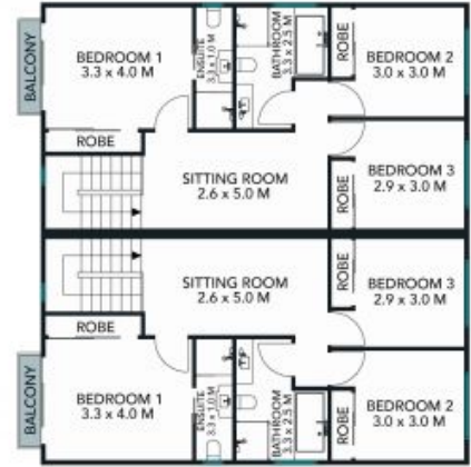
UNITS 3 & 4 SECOND FLOOR PLAN
