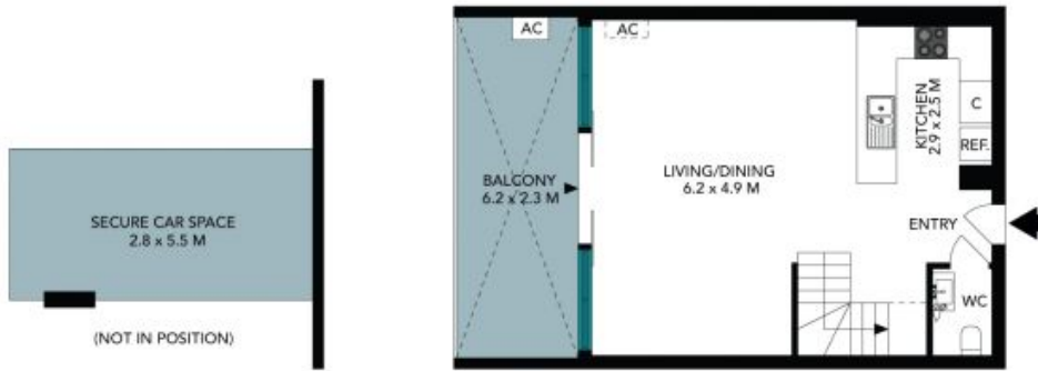
Lower Floor
