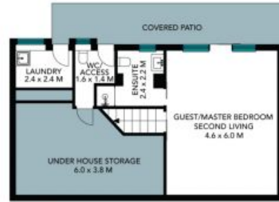
1st Floor
