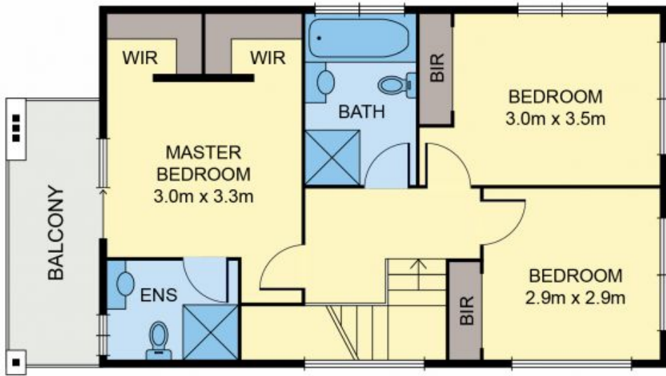
FIRST FLOOR
