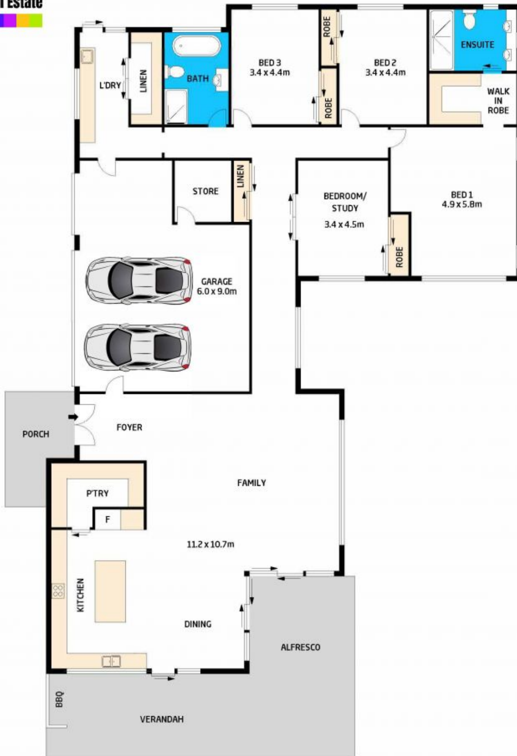
GROUND FLOOR
