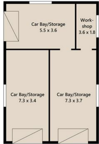
GARAGE
