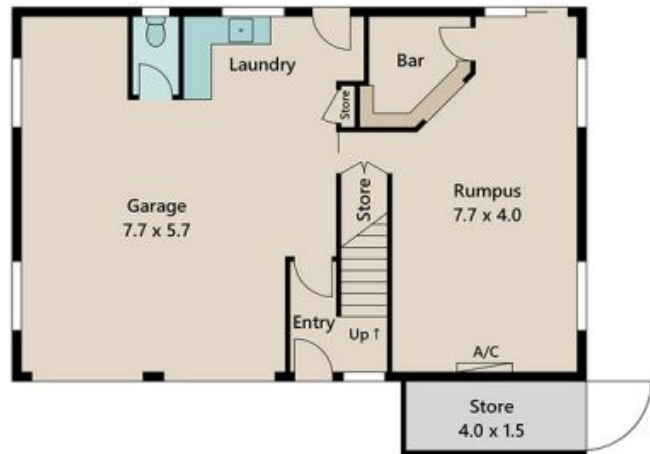
LOWER FLOOR
