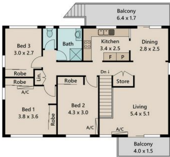
UPPER FLOOR
