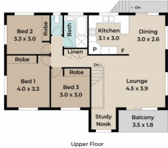
Upper Floor
