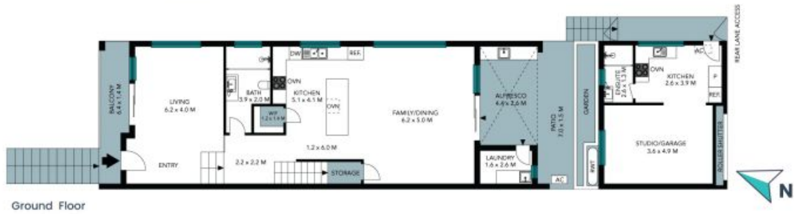
Ground Floor
