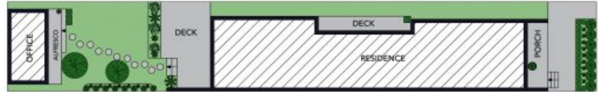
Site Plan
