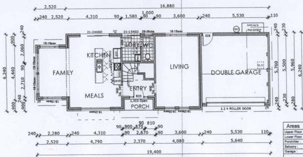
Floor Plans 1 & 2
