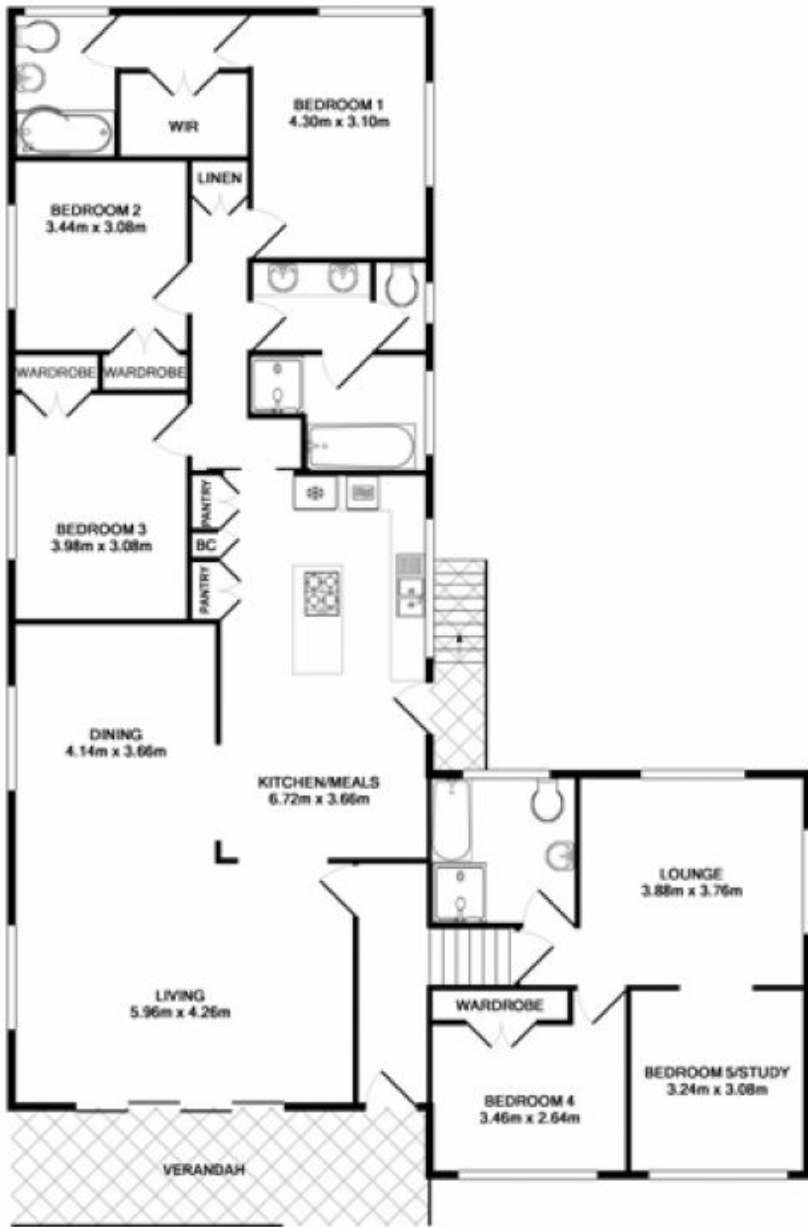
1ST FLOOR
