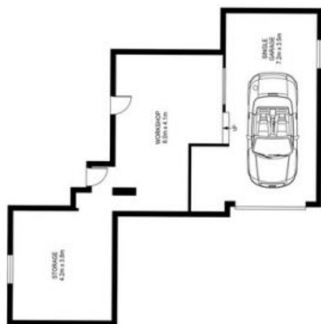
BASEMENT
