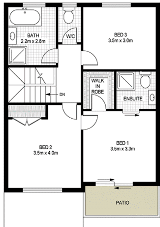
FIRSTFLOOR PLAN
