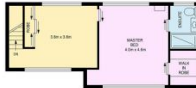
LEVEL 1 FLOOR PLAN
