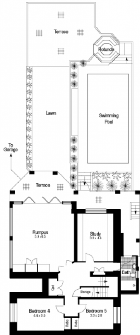
LOWER GROUND FLOOR PLAN
