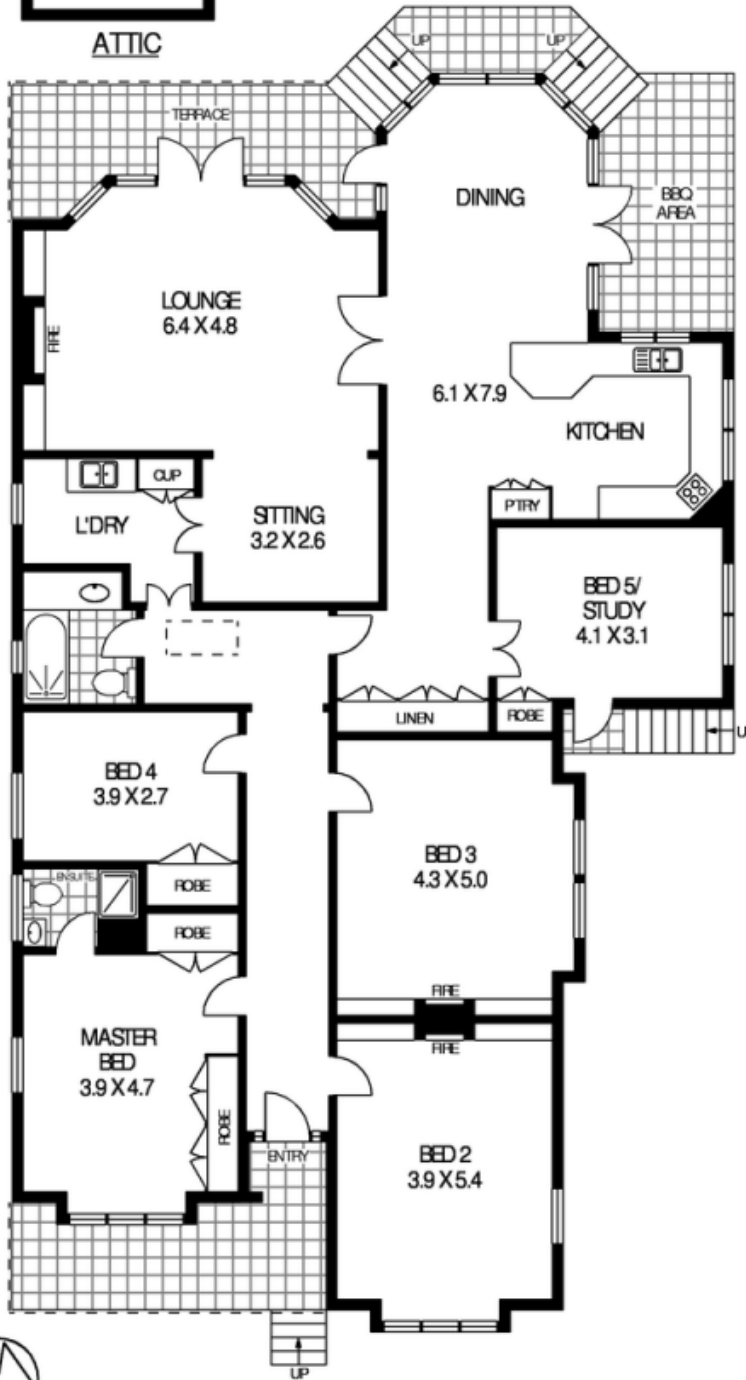
GROUND LEVEL
