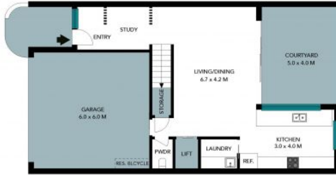
GROUND FLOOR (UNIT 5-TYPE B)
