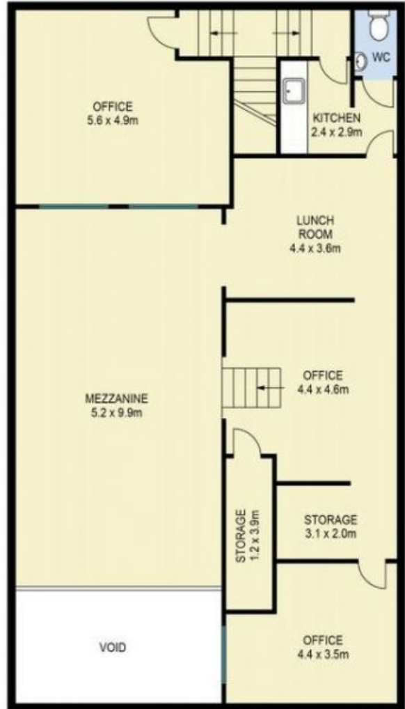
UPPER LEVEL
