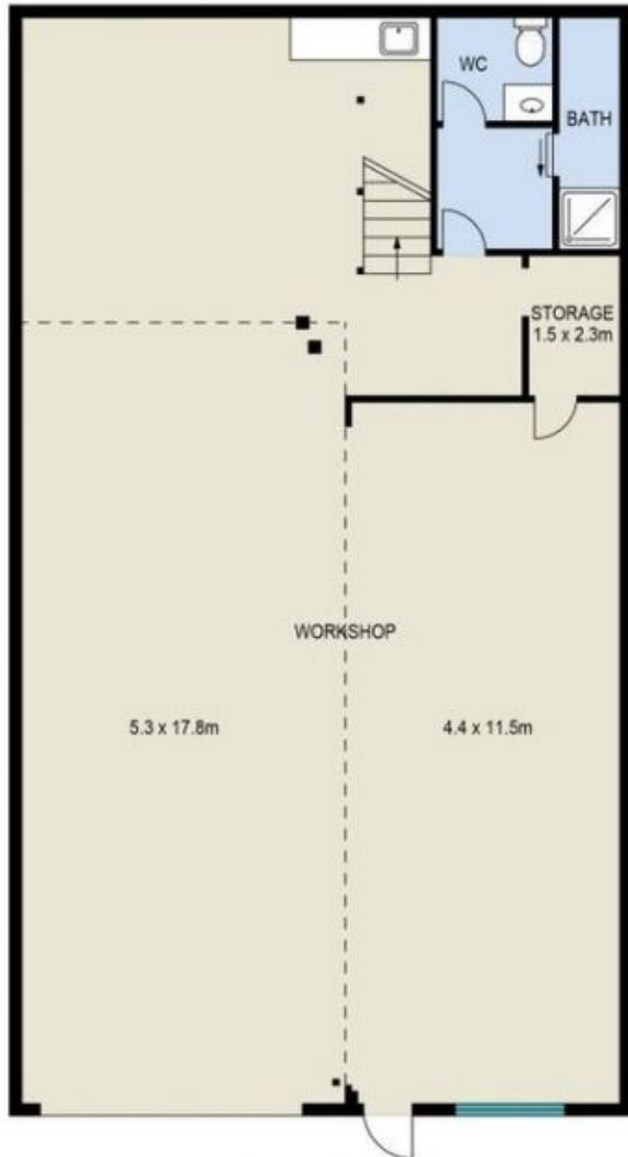
GROUND LEVEL
