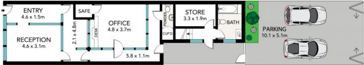
GROUND LEVEL
