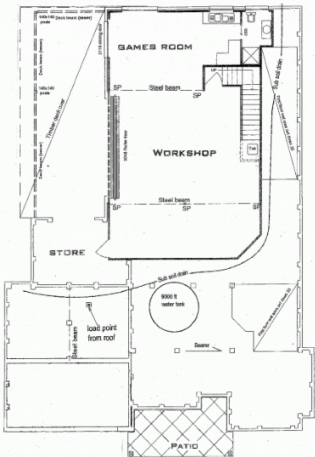
GROUND FLOOR PLAN LOT 55 WILLIAM SHARP DRIVE COFFS HARBOUR
