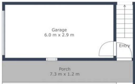
Floor 1
