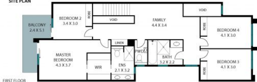
FIRST FLOOR
