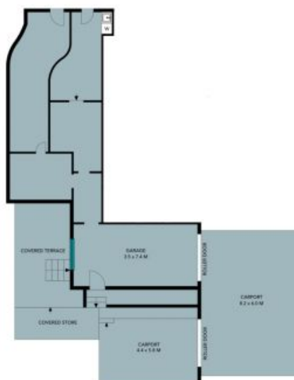
Ground Level
