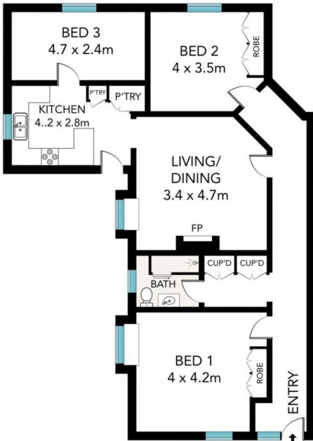
GROUND FLOOR
