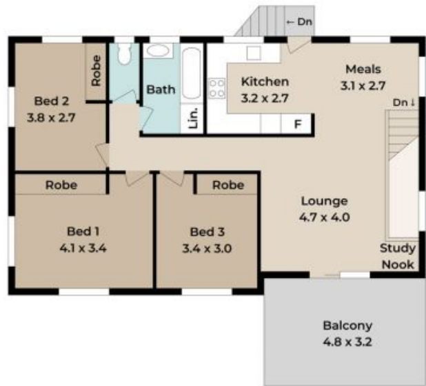
Upper Floor
