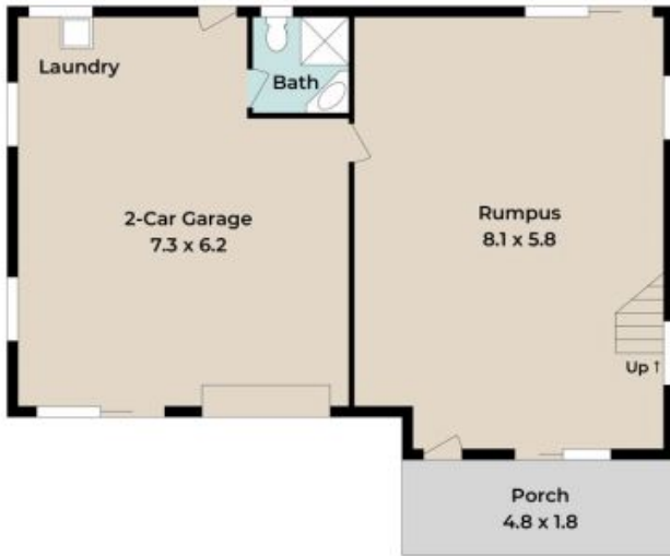
Lower Floor
